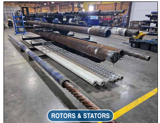
ASSORTED SIZE LOBE CONFIGURATION STATORS
