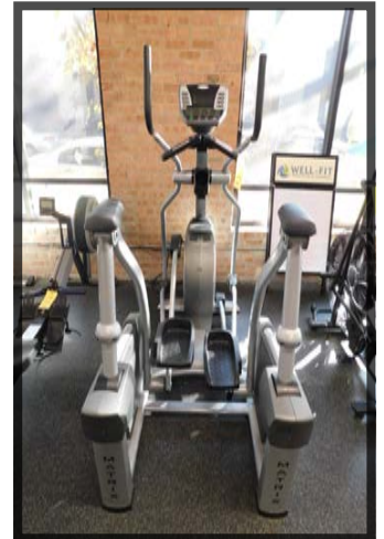
Matrix Ellipticals
