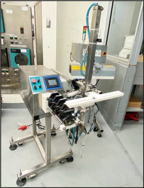
E-Z LOAD PORTABLE PLC CONTROLLED (4) TUBE PERISTALTIC BLENDER/FILLER
